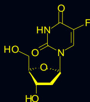
5-FLUORDESOXIURIDINA
