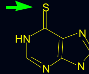
6-MERCAPTOPURINA
